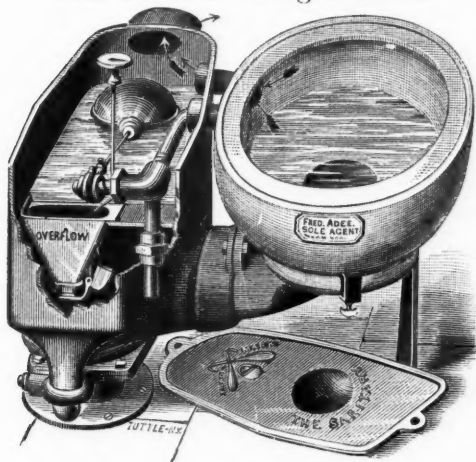
FIG. 1. STRAIGHT OUTLET.
