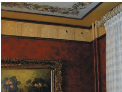
Unico's small-duct, high-velocity HVAC system takes up less than a quarter of the space of a traditional system, making it ideal for historic buildings.
