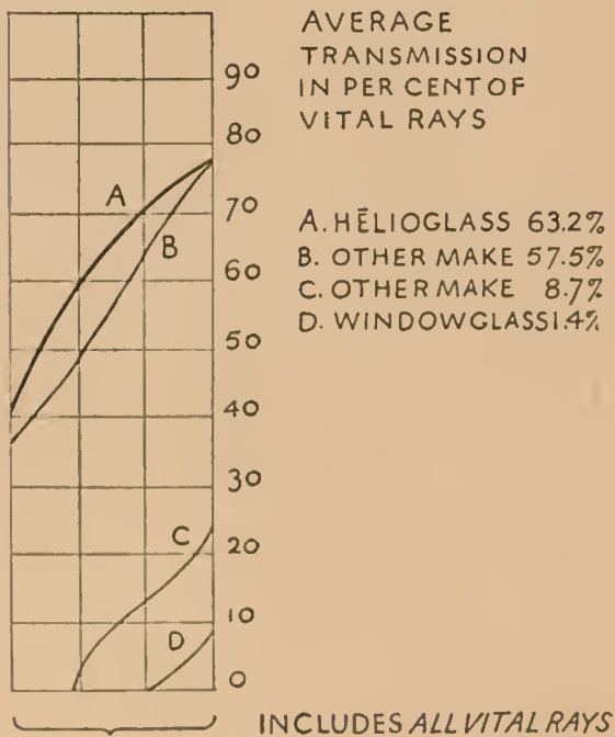
CHART INDICATES TRANSMISSION OF ULTRA-VIOLET RAYS THROUGH HĒLIOGLASS AS COMPARED TO SEVERAL OTHER MAKES AND ORDINARY WINDOW GLASS—FROM U.S. DEPARTMENT OF COMMERCE REPORT.
