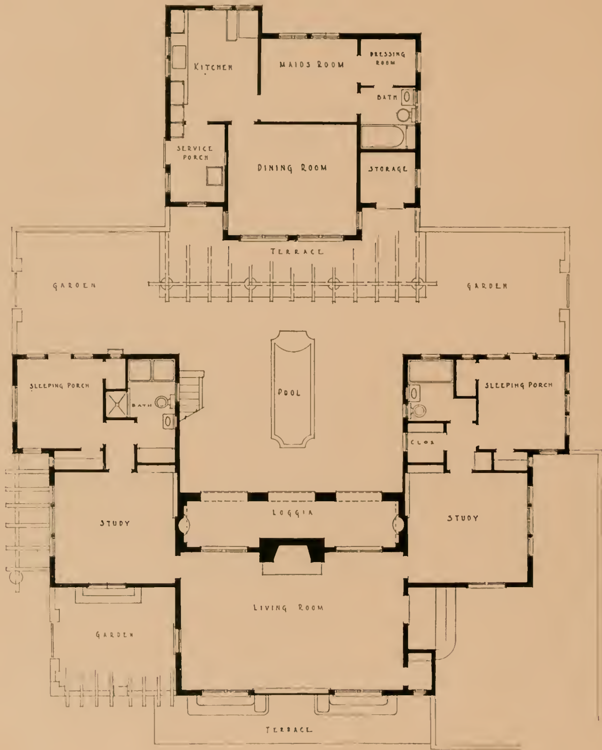
FLOOR PLAN, HOUSE OF MR. WARRINGTON, OJAI, CAL. ROBERT STACY-JUDD, ARCHITECT
