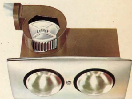
9425F 2-Bulb Heat-A-Vent® Double-duty fixture Quick radiant heat plus ventilation. Provision for 1 or 2-bulb operation. 1706 BTU – 70 CFM – 4.5 sones.
