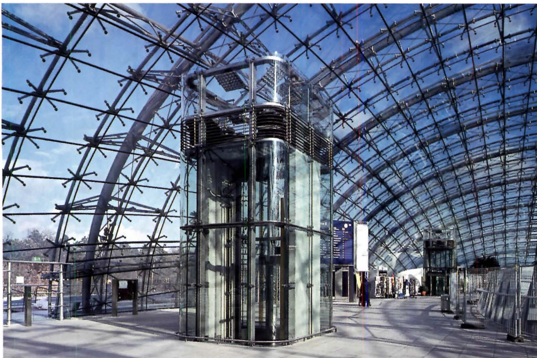
Tubular ribs frame the ticketing-level bubble (above) from the exterior (right), supporting armatures that attach glass by bolt-through connections.
