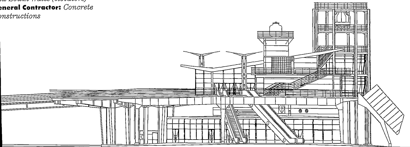
SOUTH ELEVATION
