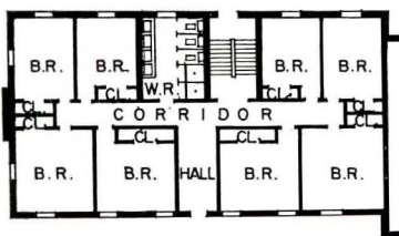
Women's dormitory, University of Maryland — nine connected four-floor units; capacity 488. Sketch shows typical living unit. Architect: Ted Englehardt. This plus a dormitory for 448 men by Mr. Englehardt and another for 368 men by Walton and Madden (see page 242) cost $2,350,000, for lowest per-bed cost in HHFA program. For all three: average area per occupant, 156 sq ft; study-bedroom, 100 sq ft; toilet-shower, 13 sq ft
