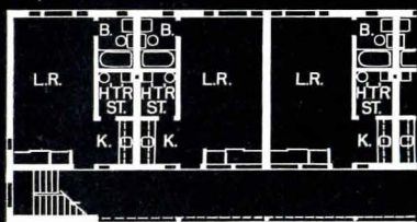
FIRST FLOOR 0 BEDROOM UNITS
