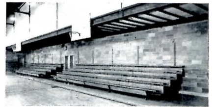
Long Island Jack Knife Bleachers, supported by steel bearing plates, fold away. Long Island Bleacher Co., Inc., 33-35 Ninth St., Long Island City 6, N. Y.
