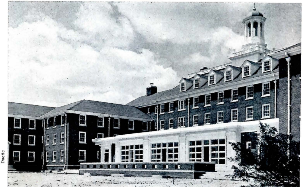
Top: men's dormitory, Colorado A & M — four three-story dormitory wings with central two-story lounge-dining unit; capacity 400, cost $1.5 million, area per occupant 248 sq ft; architect, James M. Hunter. Above: women's dormitory, Upper Iowa University — two one-story L-shaped wings joining central high-ceilinged lounge; capacity 54, cost $238,000, area per occupant 265 sq ft; architect, William A. Lockard. Below: men's dormitory, Tufts College (Mass.) — three- and four-story, includes dining facilities; capacity 280, cost $1,065,000, area per occupant 239 sq ft; architect, Arland A. Dirlam
