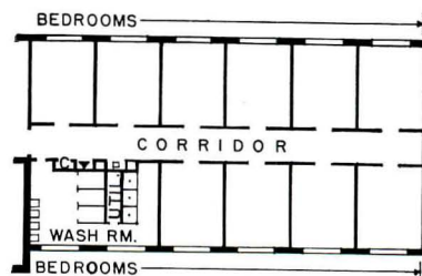
Women's dormitory, University of Southern Illinois — three connected four-story units, dining facilities included; capacity 422, cost $2,059,000. Sketch: typical living arrangement in one unit; lounge adjoins with another 12 bedrooms beyond. Total area per student, 255 sq ft; study-bedroom per student, 90 sq ft; toilet-shower per student, 12 sq ft. Architects: Shaeffer, Hooton & Wilson
