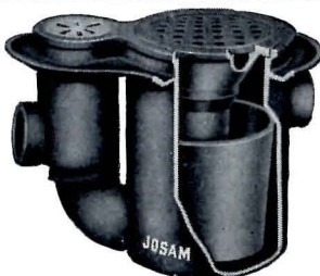
11 Josam Series No. 6800 Floor Drain with funnel shaped seal, sediment bucket and floor clean-out, for intercepting oils, gasoline and other volatile liquids.
