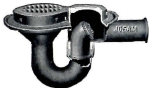
5 Josam Series No. 860-V Floor Drain with brass back water valve caulked into trap and floor cleanout.
