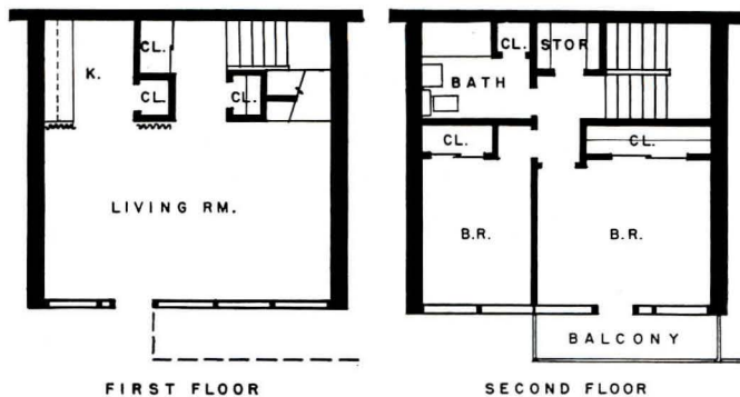
One of four separate two-story units containing a total of 92 apartments for married students and 52 for faculty at Indiana University. Total cost, $2,050,000; average area per student apartment, 615 sq ft; average area per faculty apartment, 1140 sq ft. Two of the units have duplex apartments — sketches show typical plans in this one. Architect: Edward D. James
