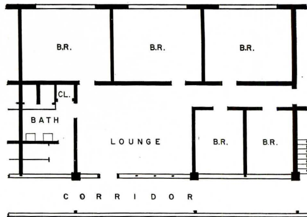
Two men's dormitories for Menlo (Junior) College (Cal.) — two-story units provide for 128 students and eight faculty apartments; cost $520,000. Typical living arrangement (sketch) provides lounge and washroom for each eight students. Area per student, 204 sq ft; study-bedroom per student, 107 sq ft; toilet-shower per student, 15 sq ft. Architect: Kingsford Jones
