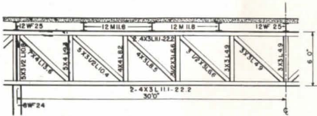
20'0" X 60'0" BAY
