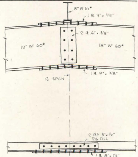
100' TIED ARCH DESIGNED FOR 50* PER SQ. FT. (30*LL - 20*DL) AT 20' CENTERS
