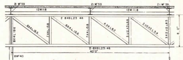
30'0" X 80'0" BAY
