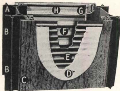
Cutaway section of Metlwal : (A) steel studs for partition, (B) snap-on indent, (C) steel panel face, (D) asbestos lining, (E) and (F) corrugated steel backing, (G) panel stiffener, and (H) 3½-in. air space
