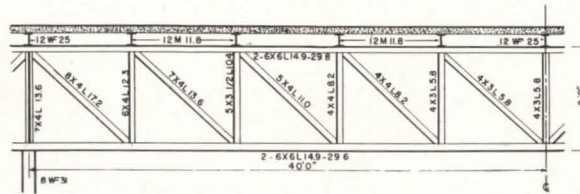
20'0" X 80'0" BAY
