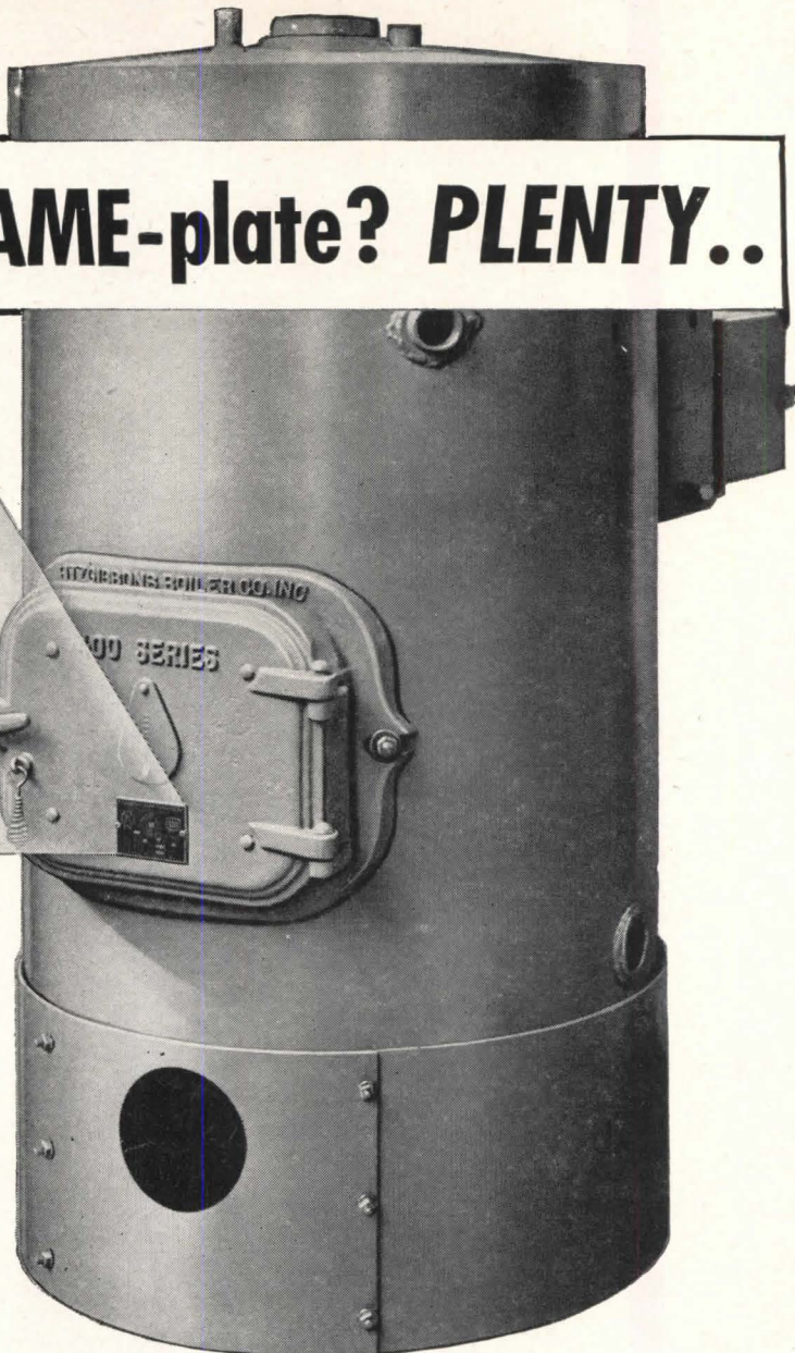
This is the bare boiler without trim or insulation. The quickly attached jacket, now available, covers and protects everything including burner and all controls.
