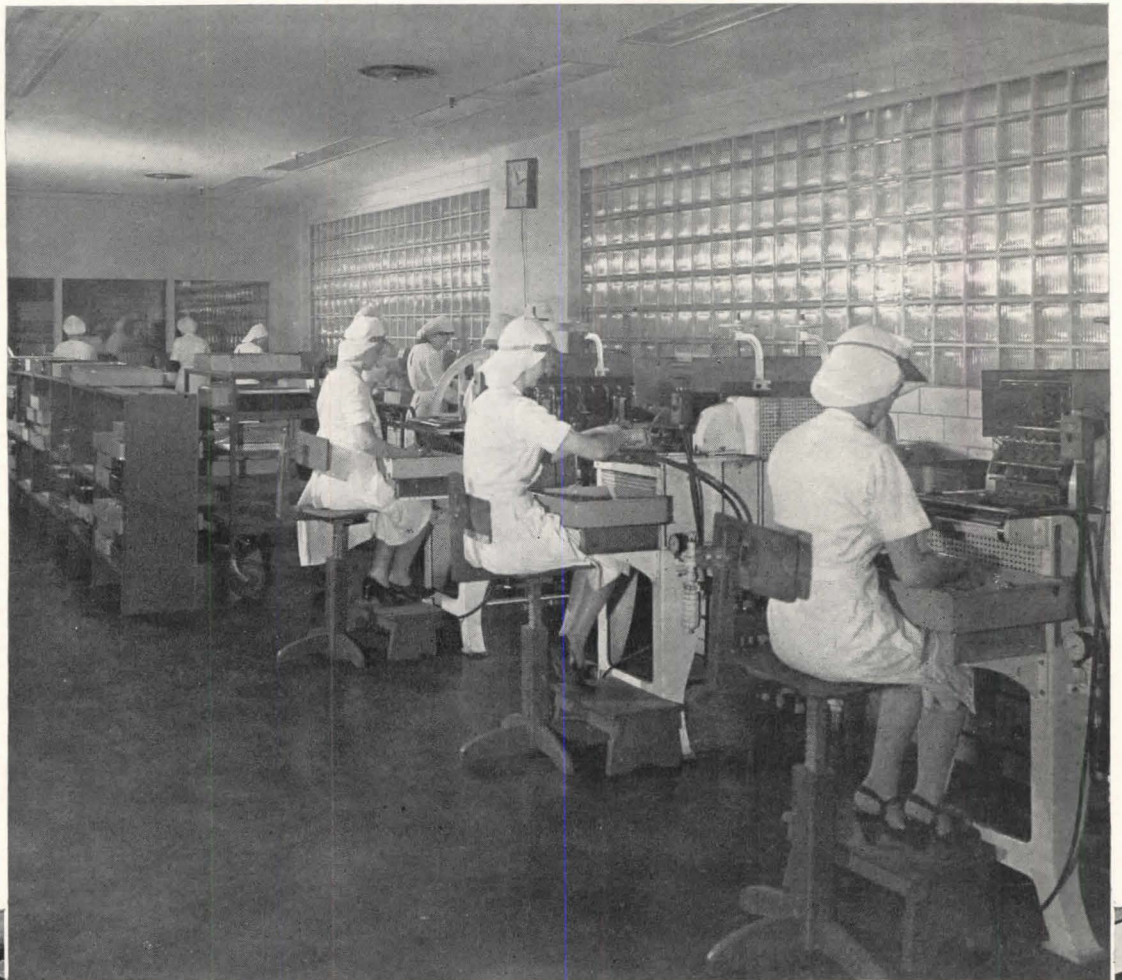
Below: immaculate conditions must be maintained where ampuls, vials and bottles are washed. Bottom, left: air washers and refrigerating compressors. Bottom, right: control center for compressors, dust-collecting and vacuum
