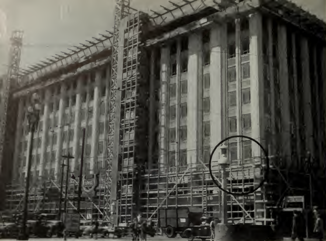
CERAMIC VENEER (TERRA COTTA) ADHESION TYPE: All plain areas are one-inch thick Ceramic Veneer applied by adhesion of the three-quarter-inch mortar coat. Anchors are used in the heavy ornamented courses only.
