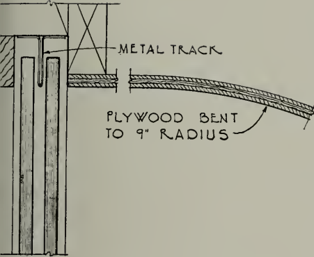
PLAN THROUGH DISPLAY SHELF
