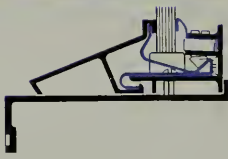
✦ EXTRUDED SASH
