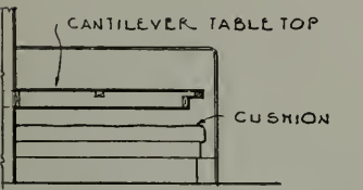
SECT. THROUGH BOOTH SCALE 1/4" = 1'-0"
