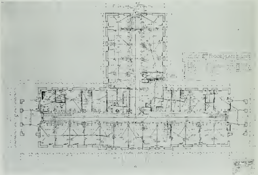
SECOND FLOOR PLAN, L. D. S. HOSPITAL, IDAHO FALLS, IDAHO H. Newton Thornton, Architect
