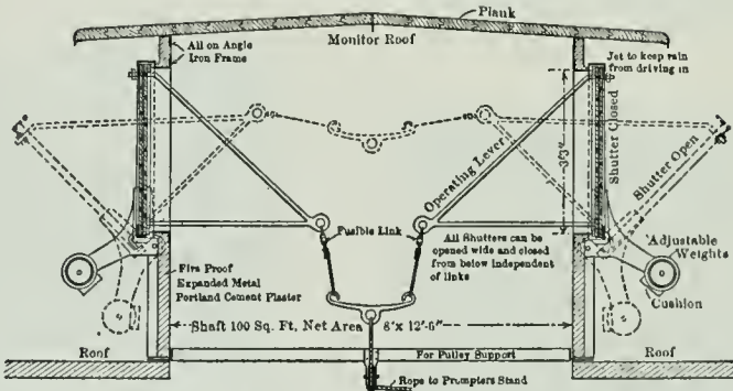
SMOKE VENT. MONITOR TYPE VERTICAL SECTION
