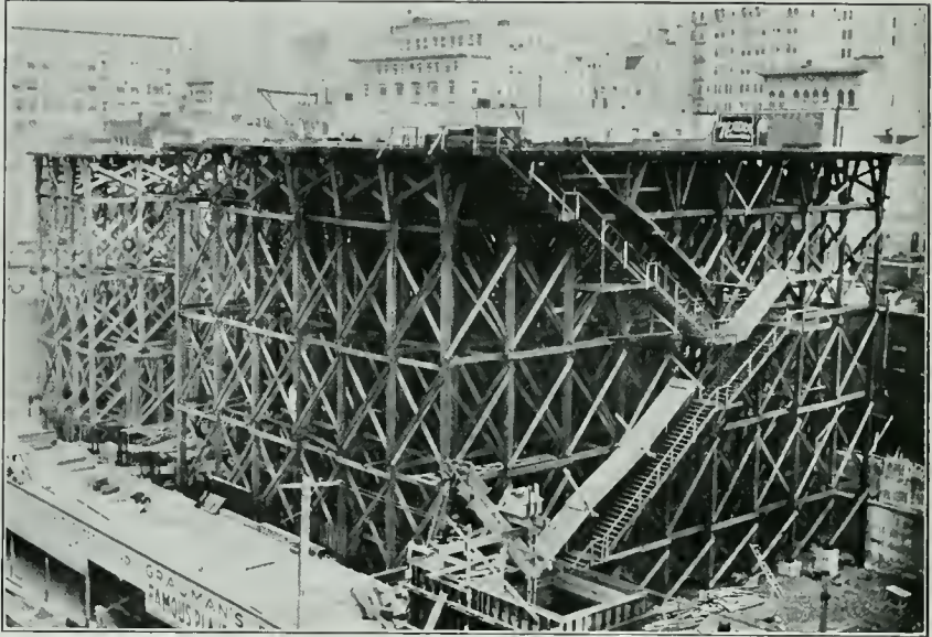
FALSE-WORK USED TO CARRY LARGE REINFORCED CONCRETE TRUSSES, GRAUMAN'S THEATER, LOS ANGELES
