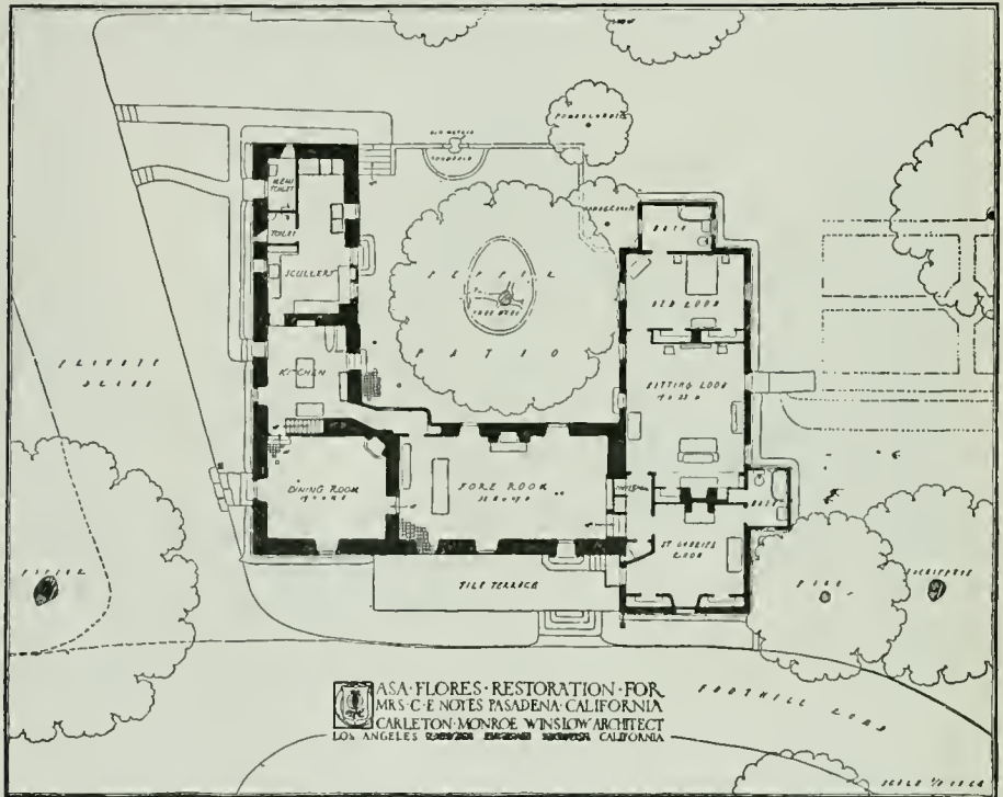
CASA FLORES. RESTORATION FOR MRS. C. E. NOYES, PASADENA, CAL. Carleton Monroe Winslow, Architect.
