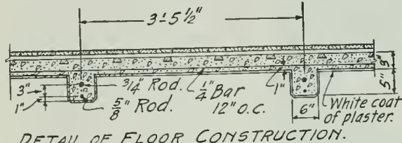
DETAIL OF FLOOR CONSTRUCTION.
