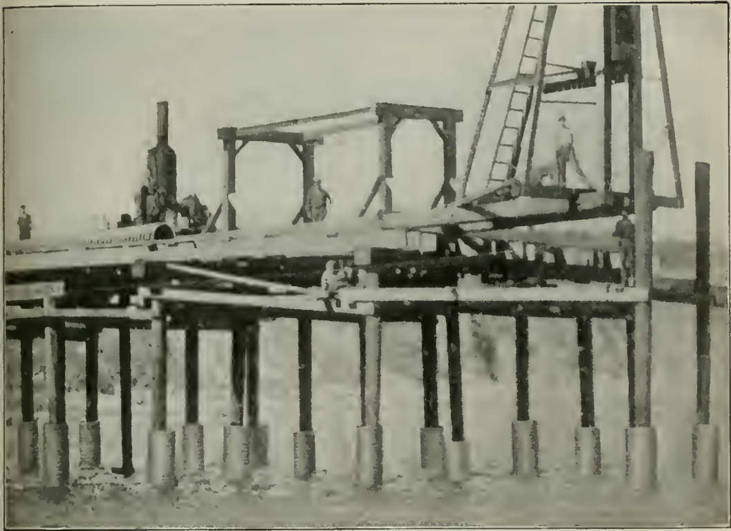
Fig. 3—A close-up view of the wharf recently constructed by the port of Port Orford, Curry County, Oregon, showing how ingot iron corrugated pipes were installed to prevent attacks by marine woodborers.
