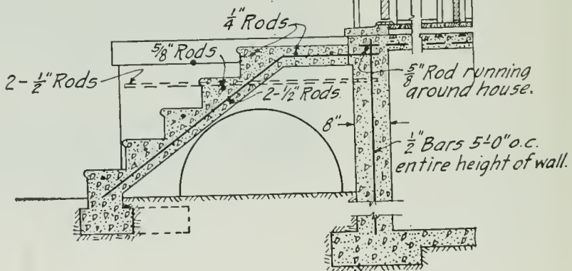
CROSS SECTION OF WALL.
