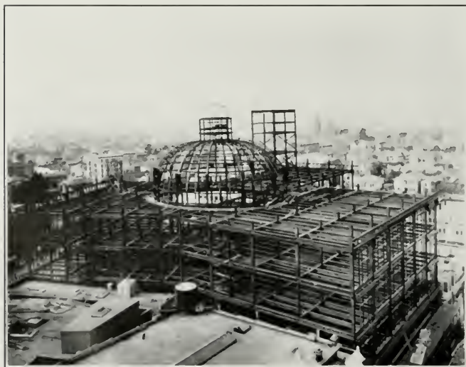
Steel Frame, Kohn Building, Oakland C. W. Dickey, Architect
