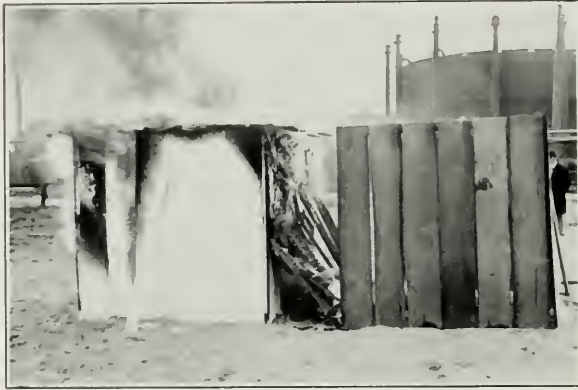
Fig. 2, Showing Fall of Unpainted Wall Against Painted One
