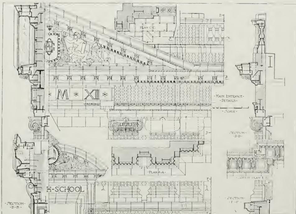
Lecca Cotta Details, Girls High School Building San Francisco
