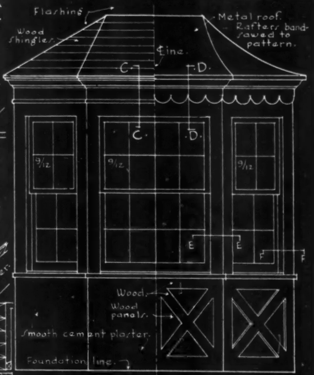
HALF ELEVATION
