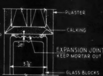
HEAD DETAIL "G"
