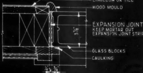
JAMB DETAIL "D"
