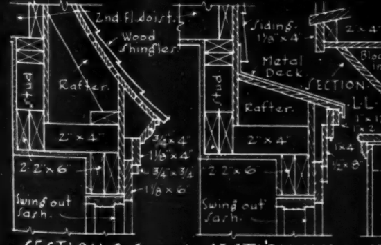
SECTION G-G
