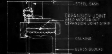
MULLION DETAIL "E"
