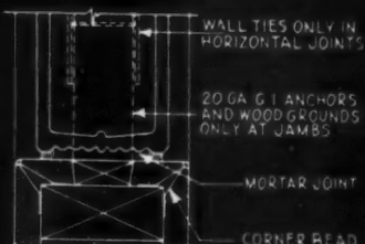
JAMB DETAIL "J"
