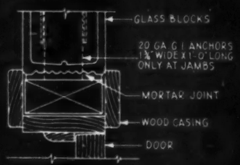
DOOR JAMB DETAIL "F"
