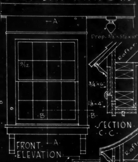
BAY UNDER 2ND STORY OVERHANG
