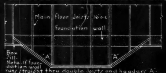
FLOOR JOIST AT RIGHT ANGLE TO WALL TYPICAL JOIST FRAMING
