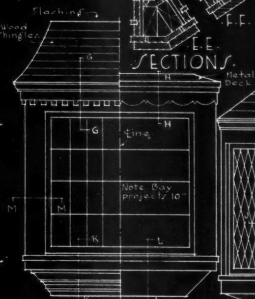
HALF FRONT ELEVATION
