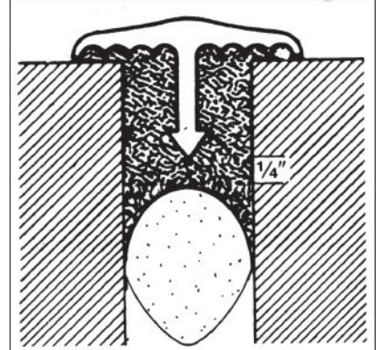
Weathercap's joint protection system is a soft-lead strip embedded in caulk to form a cap or seal for any masonry joint.
