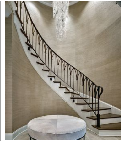
This custom designed, hand forged wrought iron staircase railing by Heritage Metalworks is intricately assembled, featuring Gothic arches and finished with a hammered texture. (Photo by Don Pearse Photography, Inc.)
