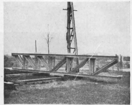
50-ft. trusses in new welded design
