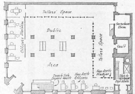
New first floor
