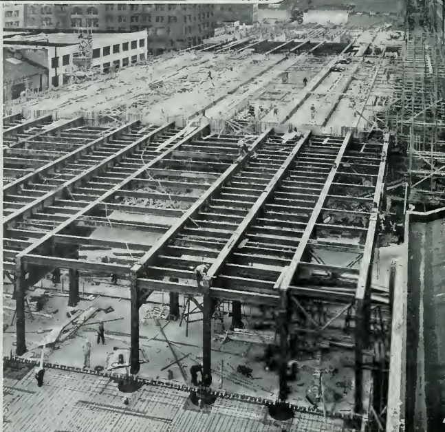
New Bay Bridge Terminal under construction. Built by the State Department of Public Works, Earl Lee Kelly, Director; under the jurisdiction of the California Toll Bridge Authority, Gov. Frank F. Merriam, Chairman, C. H. Purcell, Chief Engineer, General Contractor for Structural Steel—Columbia Steel Co.
